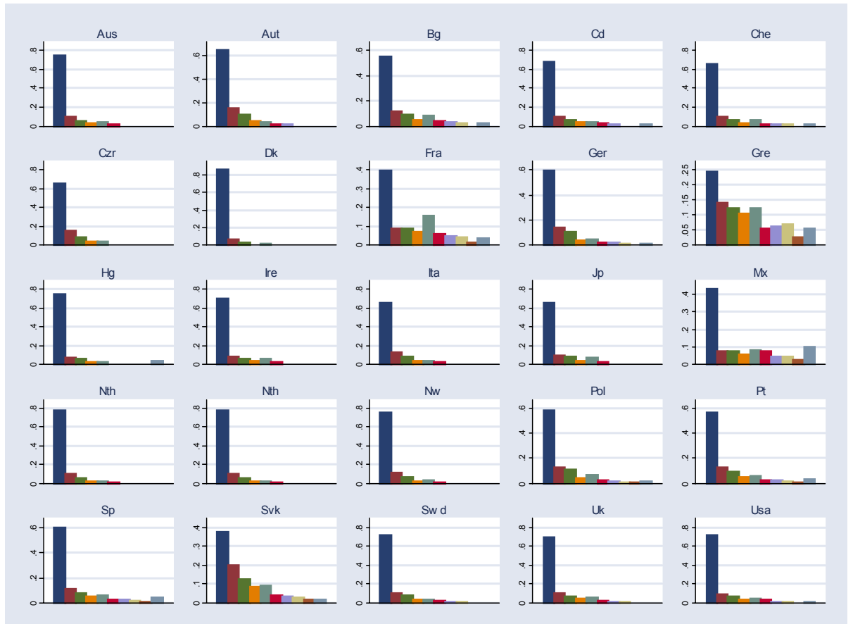
Figure 7: “Do you think it can always be justified, never be justified or something in between to claim government/state benefits to which you ave no rights”. From 1=“Never justifiable” to 10“Always justifiable”. WVS: 1981,1990, 1999-2001.
