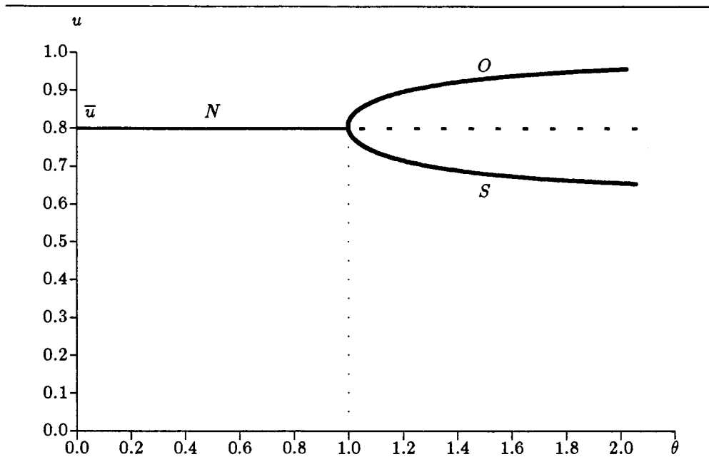
Figure 3 - The Pitchfork The Configuration of Equilibria
